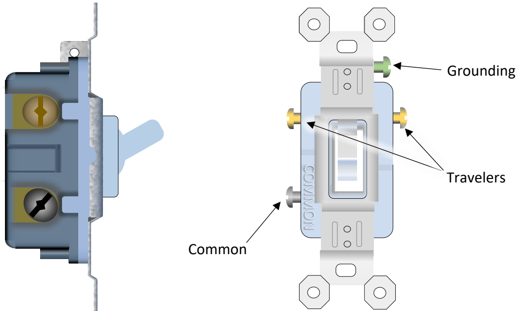
Figure 1. Front and side views of a three-way switch.
