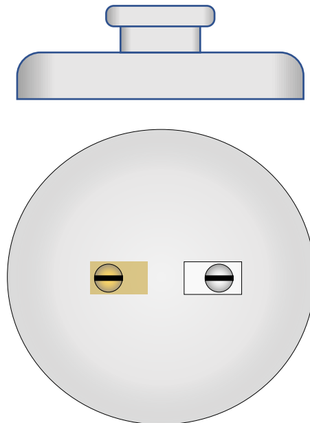
Figure 2. Front and bottom views of a light fixture.
